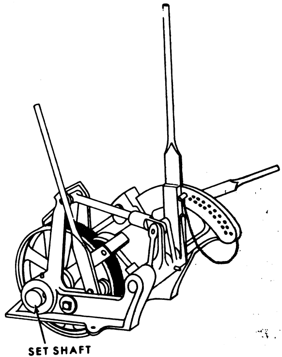
Figure 8-15. Boss dog.
